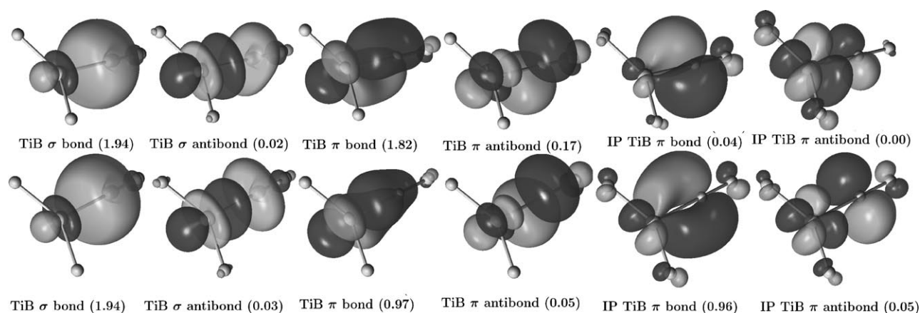
Figure 3. The active molecular orbitals in \text{FB}=\text{TiF}_2 for the singlet (top row) and the triplet states. The contour line used is 0.05 e.u. -3 . MO occupation numbers are given with each orbital.
