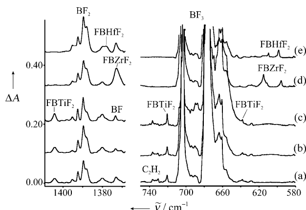
Figure 1. Infrared spectra for group 4 metal atom reaction products with \text{BF}_3 in excess argon in the 1410\text{--}1370 and 740\text{--}580\text{ cm}^{-1} regions. a) spectrum after co-deposition of laser-ablated Ti and \text{BF}_3 at 0.5 % in argon at 6 K for 60 min, b) after annealing to 20 K, and c) after > 220\text{ nm} irradiation for 20 min, d) spectrum after co-deposition of laser-ablated Zr and \text{BF}_3 at 0.5 % in argon at 6 K for 60 min, and e) spectrum after co-deposition of laser-ablated Hf and \text{BF}_3 at 0.5 % in argon at 6 K for 60 min.
