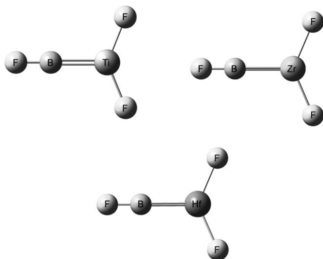
Figure 2. Structures calculated for the group 4 transition metal difluoride borylene complexes using B3LYP, BPW91, and CASSCF/CASPT2 methods. The structures are C 2v for FB=TiF 2 and FB=ZrF 2 and C 3v for FB=HfF 2 .
